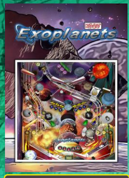
Exoplanets
